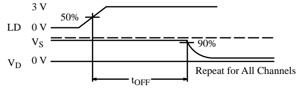
Figure 2. t_{OFF} from LD
