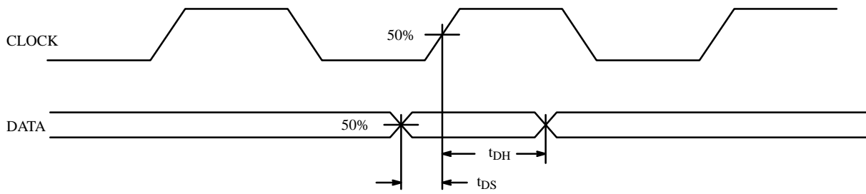
Figure 4. Data Setup and Hold Time
