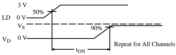
Figure 1. t_{ON} from LD
