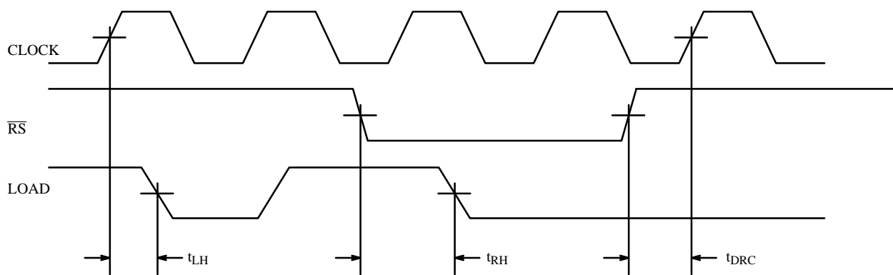
Figure 5. Timing Relationships
